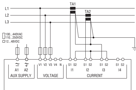
ARON connection 3-phase without neutral, whit or without V4 P01.07 = L1-L2-L3
