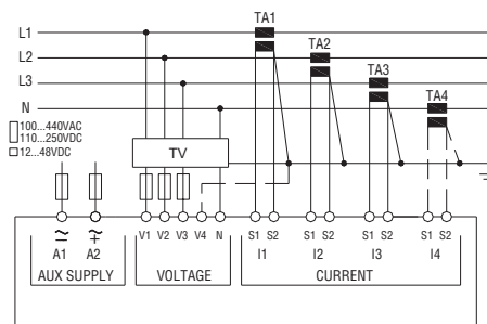
3 phase connection with neutral via VT, whit or without V4 and neutral current Set P01.04, P01.05 and P01.06 P01.07 = L1-L2-L3-N
