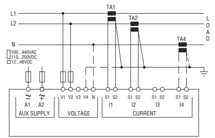
2-phase connection whit or without V4 and neutral current P01.07 = L1-N-L2
