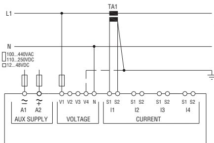
Single-phase connection whit or without V4 P01.07 = L1-N
