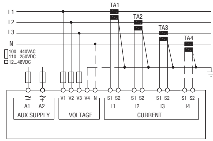
3-phase connection whit or without neutral, V4 and neutral current P01.07 = L1-L2-L3-N L1-L2-L3
