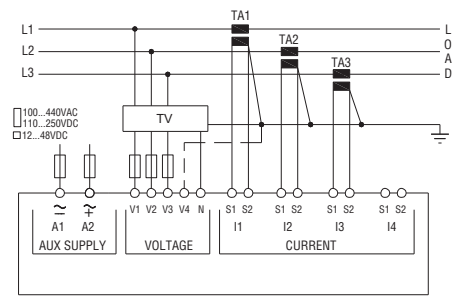
3 phase connection without neutral via VT, whit or without V4 Set P01.04, P01.05 and P01.06 P01.07 = L1-L2-L3
