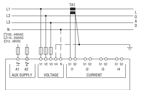
Balanced 3-phase connection whit or without neutral and V4 P01.07 = L1-L2-L3-N-BIL L1-L2-L3-BIL
